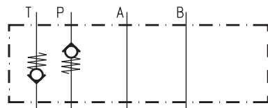
HROPT 壓力夾緊和背壓
